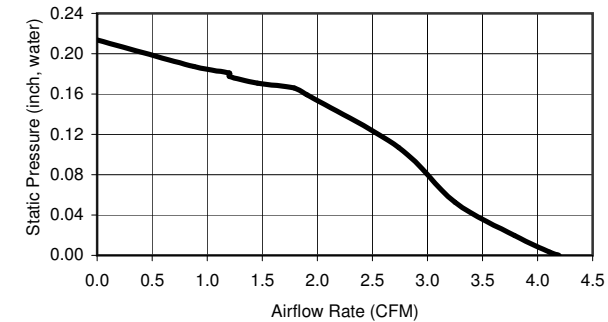
PQ CURVE
