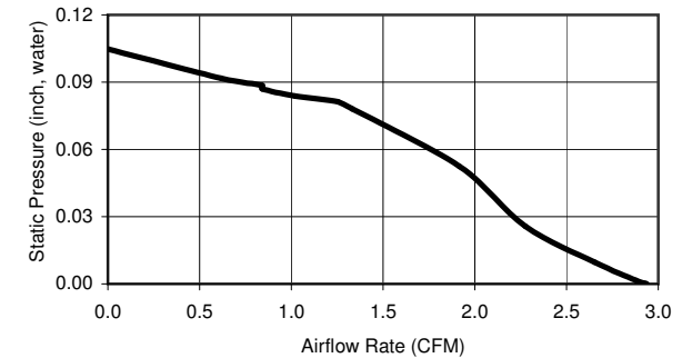
PQ CURVE
