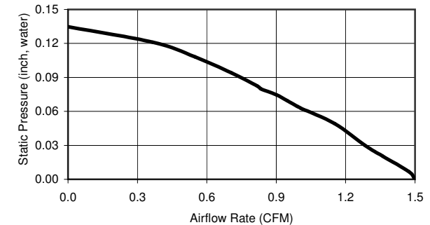
PQ CURVE
