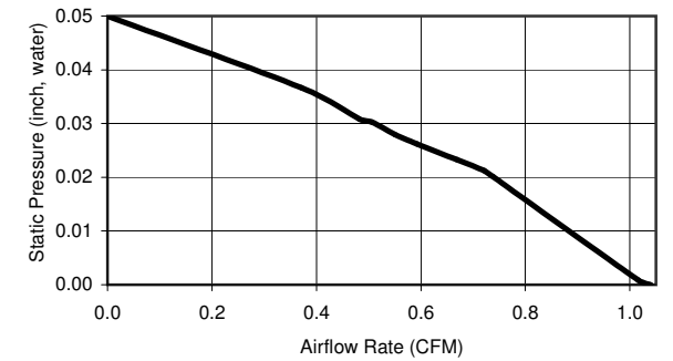
PQ CURVE
