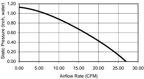
PQ CURVE
