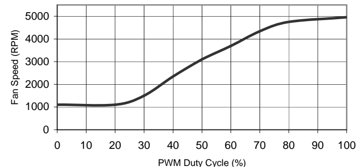
PWM DUTY CYCLE vs. FAN SPEED
