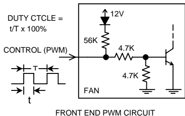
FRONT END PWM CIRCUIT
