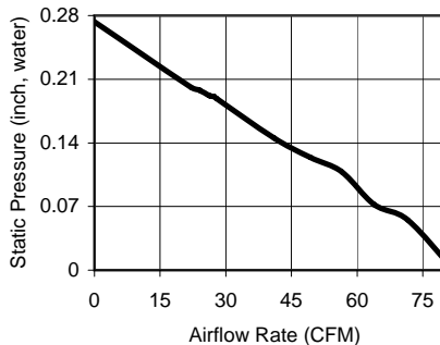
PQ CURVE
