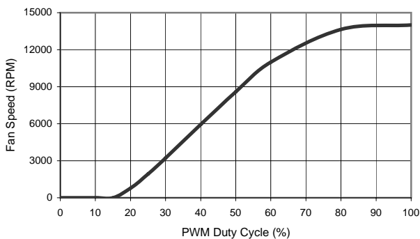
PWM DUTY CYCLE vs. FAN SPEED
